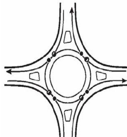
Roundabout With 12 potential points of conflict
